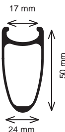
Wheel Profile
