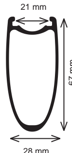
Wheel Profile
