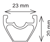
Wheel Profile
