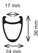
Wheel Profile
