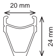
Wheel Profile
