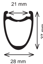
Wheel Profile
